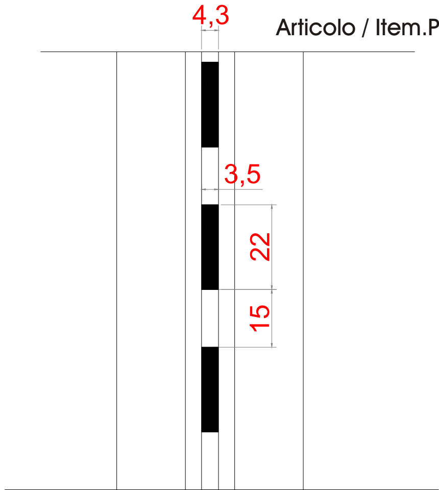
Fronte / Front
